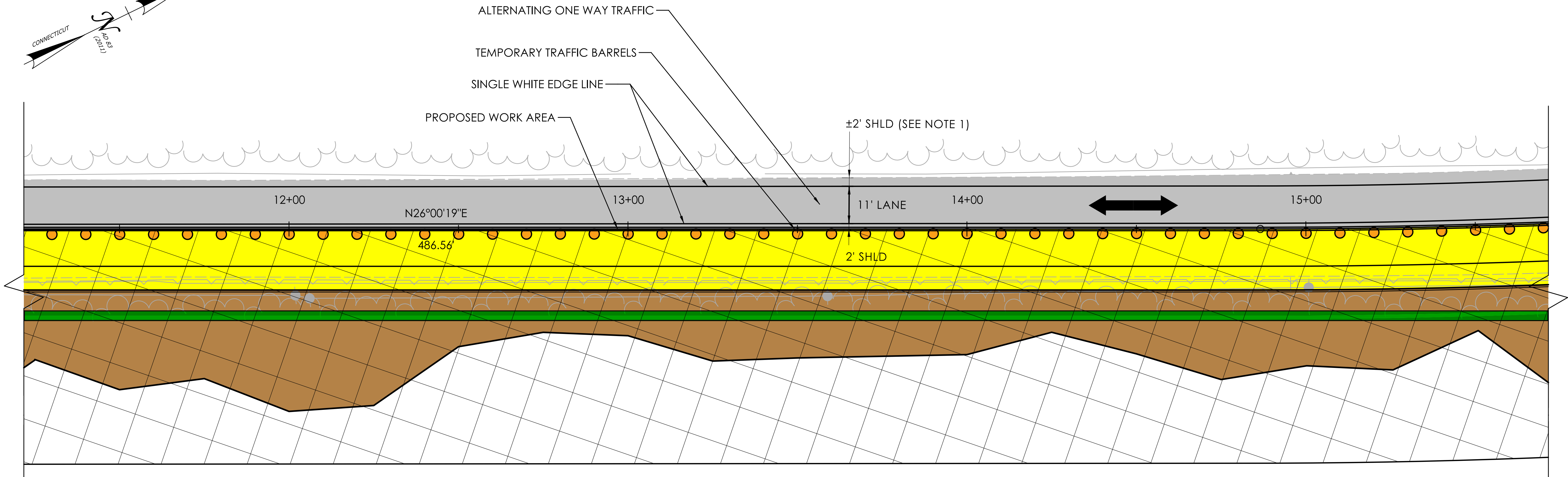
ROADWAY PLAN - DURING CONSTRUCTION
