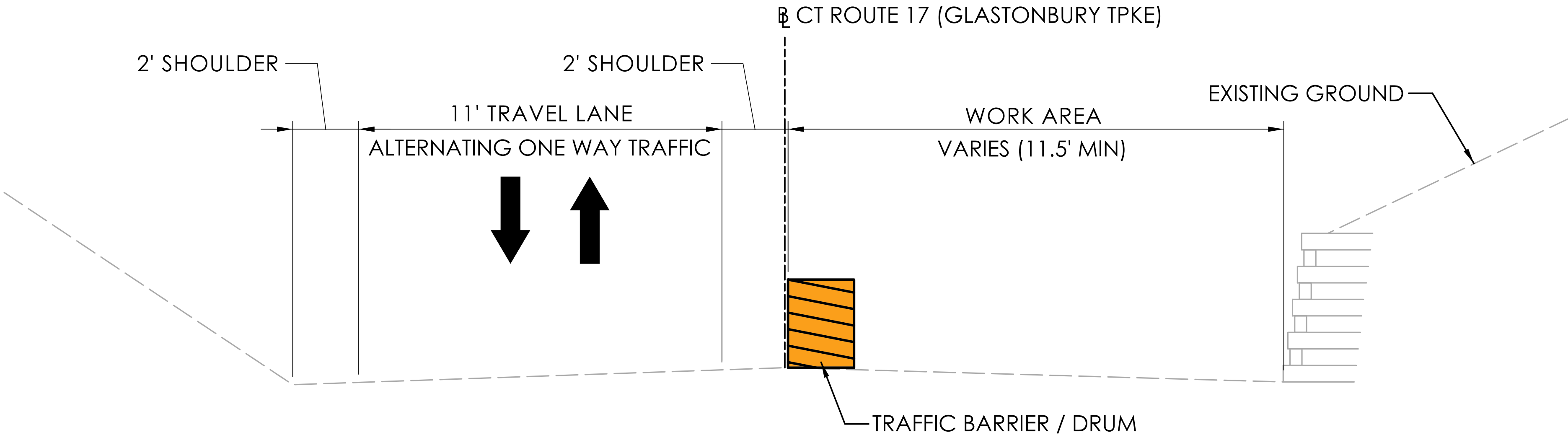
TYPICAL SECTION - DURING CONSTRUCTION (LOOKING NORTHBOUND ALONG ROADWAY)
